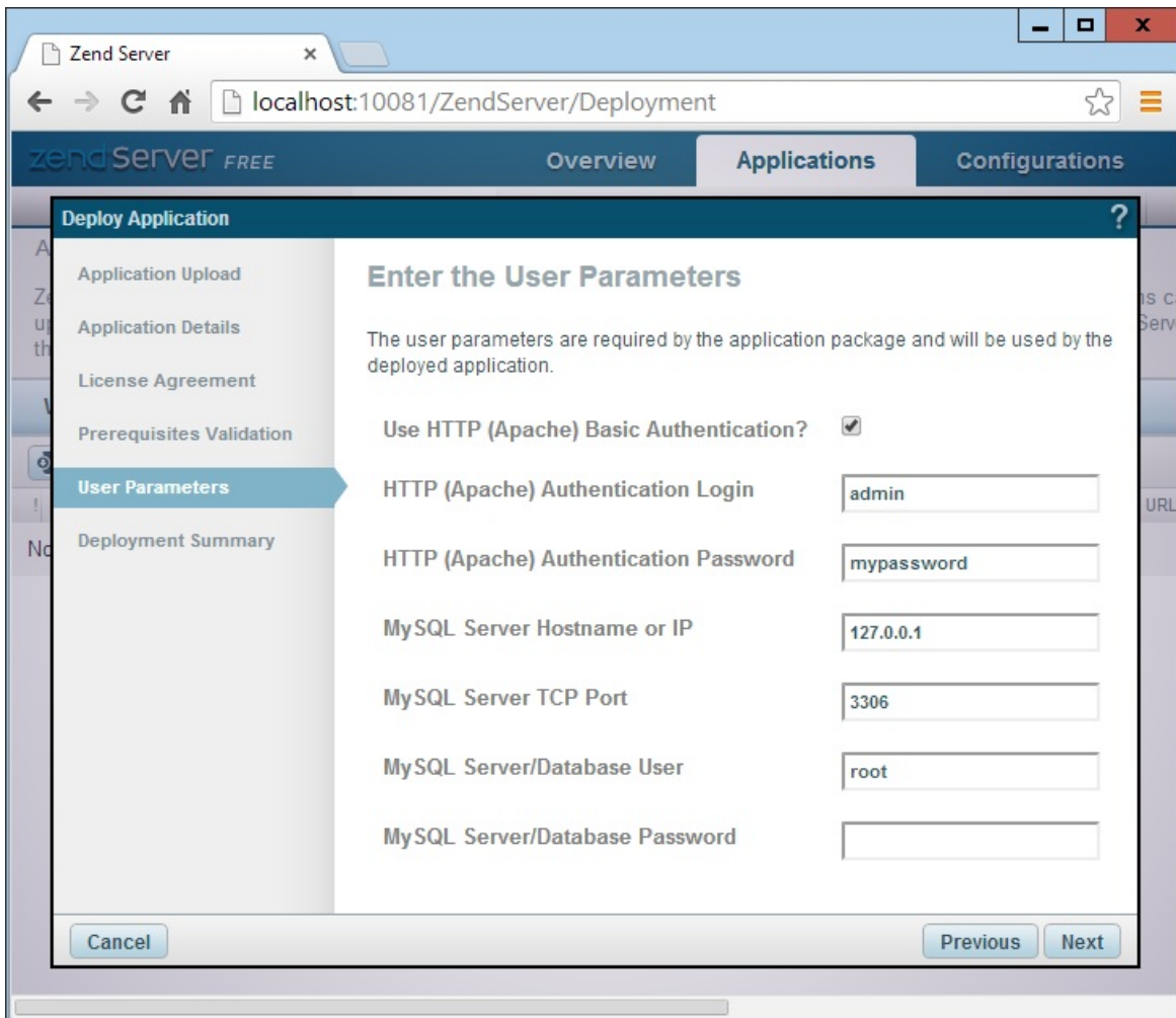
Figure 8-20. Entering phpMyAdmin user parameters
